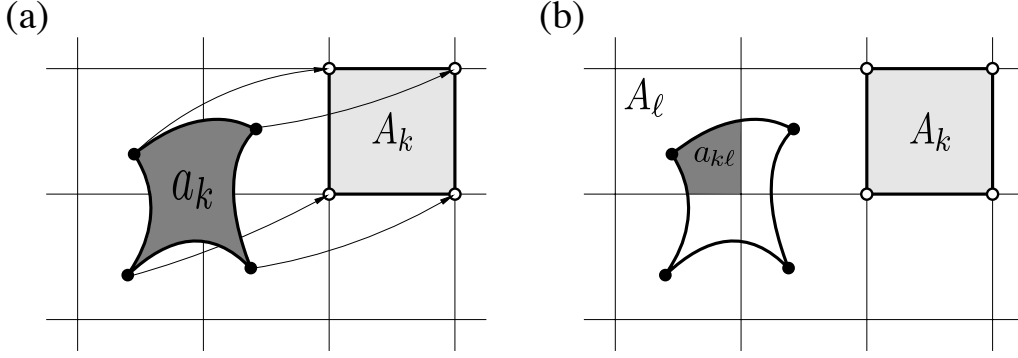
Figure 1: A schematic illustration of concepts used in the semi-Lagrangian finite-volume scheme. (a) The deformed departure cell a_k (dark shaded area) ends up, after being transported by the flow for one time-step, at the regular arrival cell A_k (light shaded area). The trajectories for the cell vertices are shown with arrows, and the departure and arrival cell vertices are marked with filled and open circles, respectively. (b) illustrates the overlap region between the grid cell A_\ell and the departure cell a_k referred to as a_{k\ell} used for the upstream integral computation given in equation (4).
