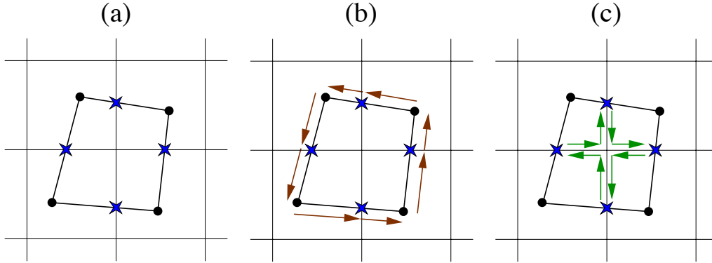
Figure 6: A schematic illustration of the search algorithm used to define the overlap regions a_{k\ell} between the departure cell (vertices marked with filled circles) and the Eulerian cells A_\ell . (a) First the intersections between Eulerian grid lines and the sides of the departure cell a_k are computed (crossings marked with stars). (b) The line segments along the sides of the departure cell a_k , referred to as outer line segments (indicated with arrows), are stored. (c) Thereafter the inner line segments along the coordinate lines and enclosed in a_k are stored (indicated with arrows).
