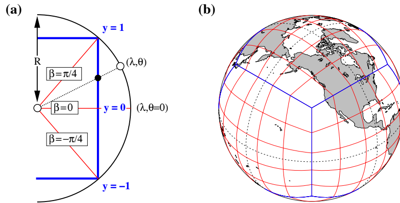
Figure 7: (a) A schematic illustration of the gnomonic coordinate. For simplicity only the y = r \tan \beta and \beta -coordinate of the gnomonic projection are shown for one of the Equatorial panels of the cubed-sphere ( \nu = 1, 2, 3, 4 ). A point on the sphere (\lambda, \theta) has the gnomonic y coordinate given by the intersection (filled circle) between face \nu of the inscribed cube (thick lines) and the straight line (dashed line) connecting the point on the sphere and the center of the sphere (unfilled circles). The central angle \beta for (\lambda, \theta) is given by the angle between the normal vector for the face and the dashed line. Solid straight lines show coordinates for the center ( \beta = y = 0 ) and edges of the panel ( y = \pm 1, \beta = \pm \pi/4 ). (b) shows the control-volumes on the surface of the sphere for the equi-angular cubed-sphere grid with N_c = 5 . Equi-angular refers to the fact that the increment in \alpha (and \beta ) for adjacent coordinate lines is constant ( \Delta\alpha = \Delta\beta ).
