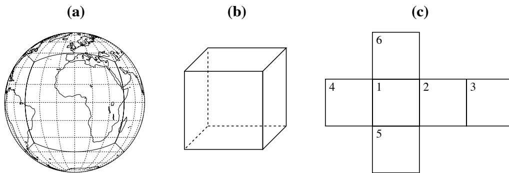
Figure 8: (a) The edges of the cubed-sphere grid plotted on the sphere (solid lines). Dashed lines show latitudes and longitudes. (b) The inscribed cube and (c) the numbering convention for the panels of the cube used in this paper. The Greenwich meridian line ( \lambda = 0 ) divides panel \nu = 1 in two.
