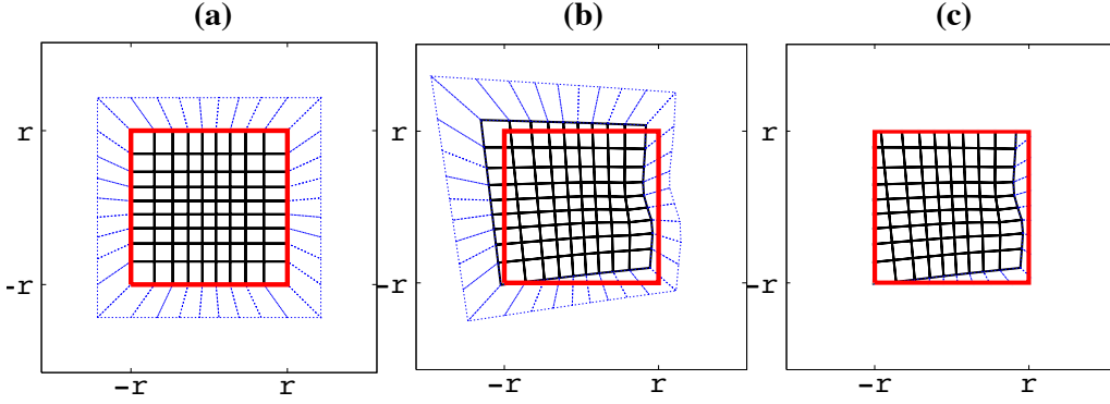
Figure 9: (a) The grid lines for panel \nu as projected onto a plane (solid black lines) and the halo zone grid lines from adjacent faces plotted on panel \nu 's projection (dashed lines). The boundary of panel \nu is marked with the thick solid (red) line. (b) The departure grid corresponding to the arrival grid shown on (a) for the moving vortices test case using a time-step of 5h. (c) The departure grid 'clipped' so it is limited to panel \nu .
