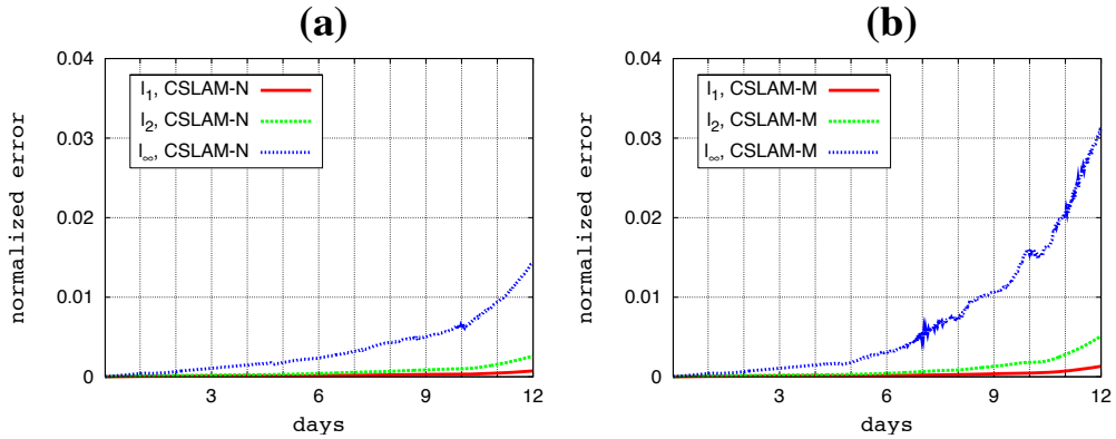
Figure 21: Time evolution of the normalized error norms ( l_1 , l_2 , l_\infty are solid, dashed and dotted lines, respectively) for the moving vortices test case with N_c = 80 (a) unlimited scheme (CSLAM-N) and (b) scheme with a monotone limiter (CSLAM-M). All settings are as in Fig. 20 and [38] (see their Fig. 12).
