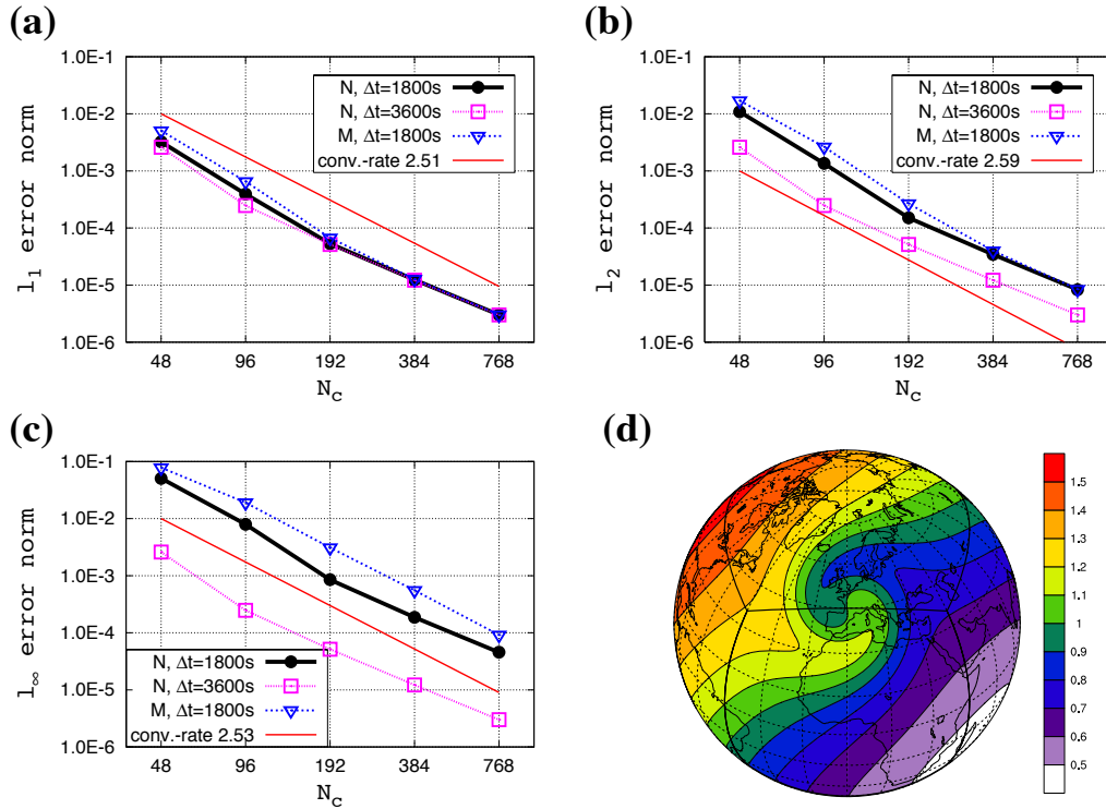
Figure 19: Same as Fig. 19 but for the moving vortices test case. Settings are as in [38] and the traditional semi-Lagrangian tests in [37], that is, \Delta t = 1800s and \Delta t = 3600s (one revolution completed in 576 and 288 time steps), respectively, and \varphi = \pi/4 . (d) shows the analytical solution after a quarter revolution.
