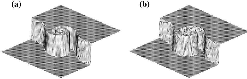
Figure 12: (a) and (b) show the exact solution and the CSLAM solution, respectively, after 16 time steps for the idealized cyclogenesis problem.
