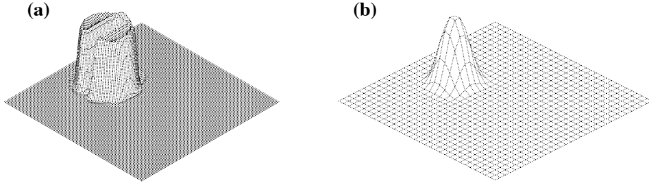
Figure 11: Surface plots of the CSLAM solution to the solid body advection of (a) a slotted cylinder and (b) a cosine hill, respectively, after one revolution.
