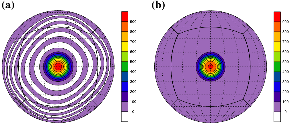
Figure 14: Numerical solution at 1.875^\circ resolution at the equator ( N_c = 48 ) for the solid body advection of a cosine hill with radius R_c = R/3 and amplitude \psi_0 = 1000 after one full revolution completed in 576 time-steps of 1800s each. (a) and (b) show the solution without and with the application of a monotone limiter, respectively. The flow is oriented with \varphi = \pi/4 so that the cosine hill passes over the edges of the cubed sphere. These settings are identical to those used in [38].
