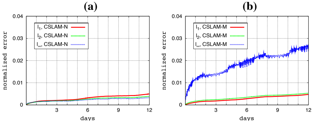
Figure 16: Time evolution of the normalized error norms ( l_1 , l_2 , l_\infty are solid, dashed and dotted lines, respectively) for solid-body advection of a cosine hill at 1^\circ ( N_c = 90 ) resolution at the equator for the (a) unlimited scheme (N) and (b) scheme with a monotone limiter (M). All settings are as in [38] (see their Fig. 3), that is, the hills radius is R_c = R/3 , its amplitude is \psi_0 = 1000 , the time-step is \Delta t = 1800s and the rotation angle is \varphi = \pi/4 so that the hill passes over four corners of the cubed sphere. One full revolution is completed in 576 time-steps.
