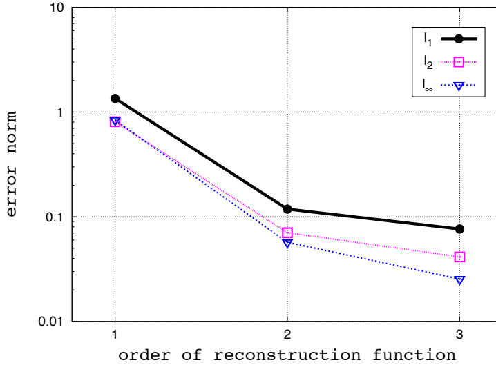
Figure 13: Standard error norms for the solid-body advection of a cosine hill for different orders of reconstruction function. Settings are as in Table 4.
