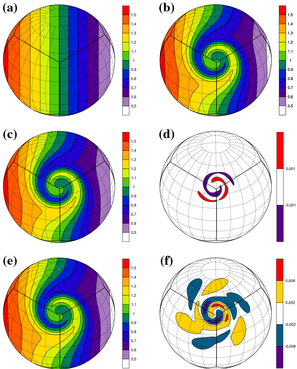
Figure 17: Results for static vortices test case. (a) shows the initial condition and (b) the analytic solution at day 6. (c) and (e) are the numerical solutions at resolutions 1.125^\circ ( N_c = 80 ) and 2.8125^\circ ( N_c = 32 ) at the equator, respectively. (d) and (f) are the corresponding plots with differences between the exact and numerical solutions.
