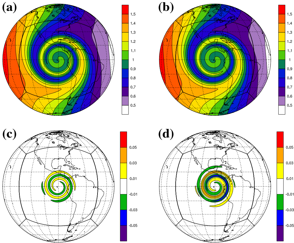
Figure 20: (a) and (b) show the CSLAM-N and CSLAM-M solutions for the moving vortices test case after one revolution, respectively, with settings as in [38] ( \varphi = \pi/4 , equatorial resolution 1.125^\circ ( N_c = 80 ), \Delta t = 1800s and 576 time-steps for one revolution). (c) and (d) are as (a) and (b) but for the difference between the numerical and exact solutions.
