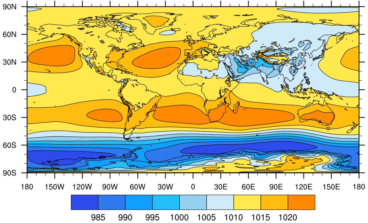
mean sea level pressure (JJA climatology)
