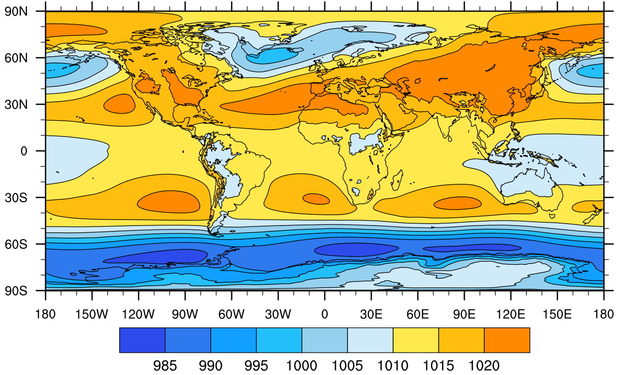
mean sea level pressure (DJF climatology)
